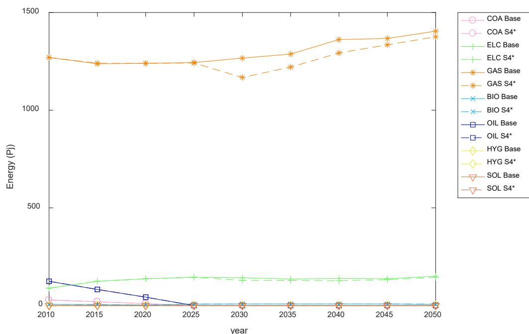
Figure 31. Fuel use for residential heating for the base scenario and S4*.
