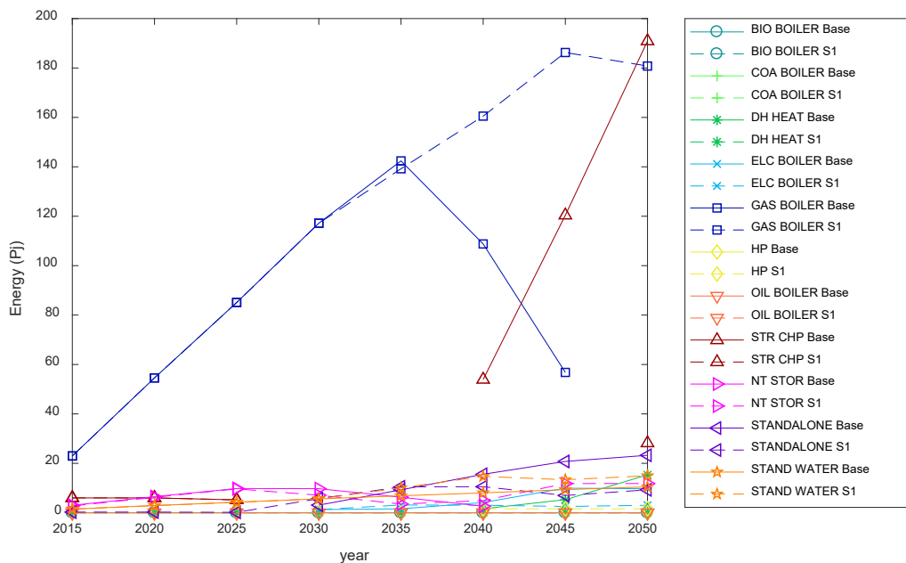
Figure 13. Production of residential heating technologies in new houses for the base scenario and S1.
