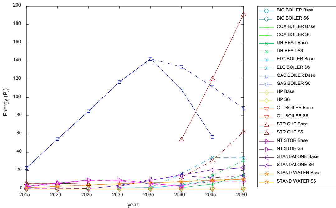
Figure 38. Production of residential heating technologies in new houses for the base scenario and S6.
