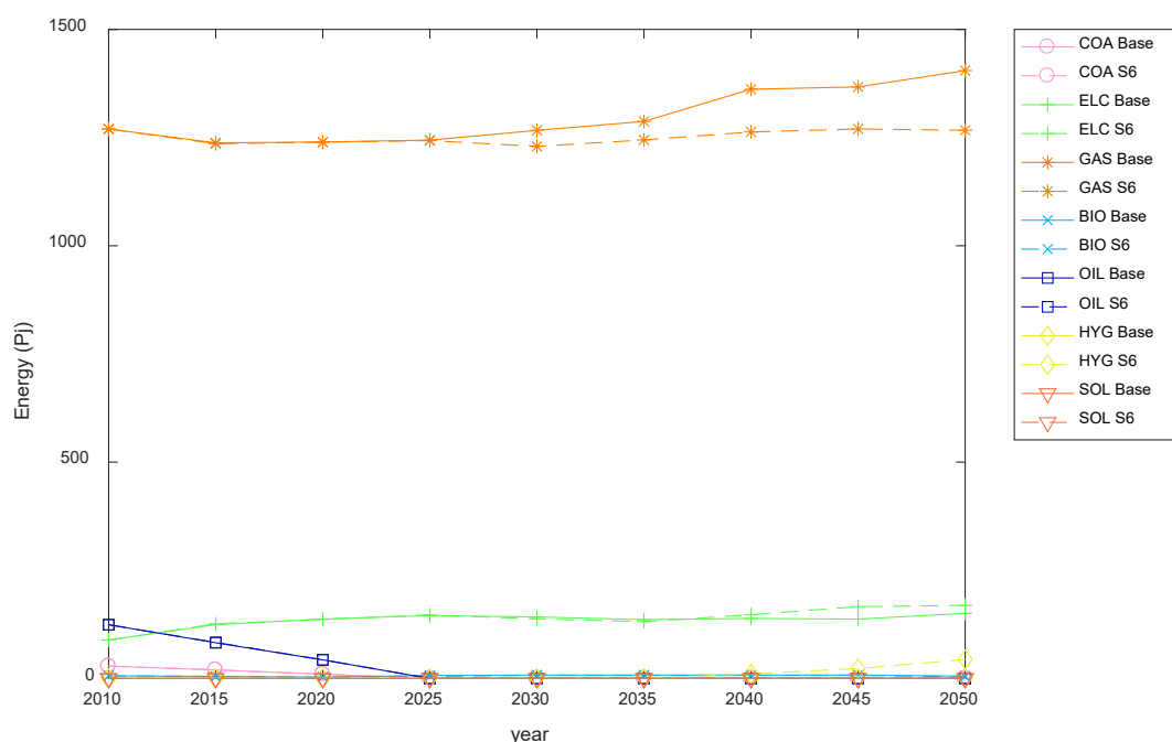
Figure 41. Fuel use for residential heating for the base scenario and S6.
