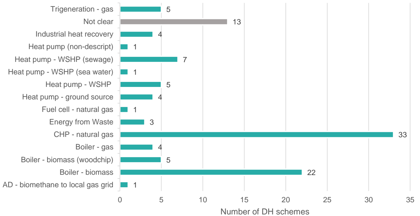
Figure 6 DH schemes by primary heating technology
